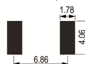
Solder Pad Layout
